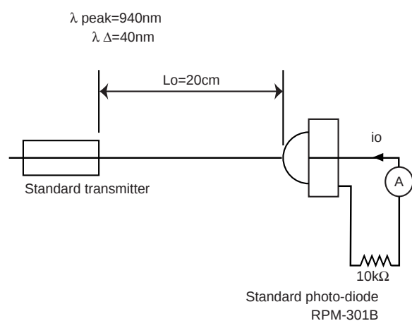
Fig.2 Measurement of standard transmitter proofreading
