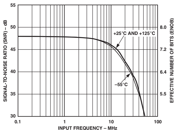
Figure 7. Dynamic Performance vs. Analog Input Frequency
