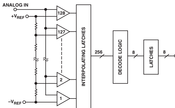
Figure 1. Comparator Block Diagram
