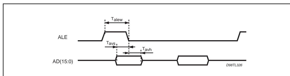
Figure 14. Waveforms
