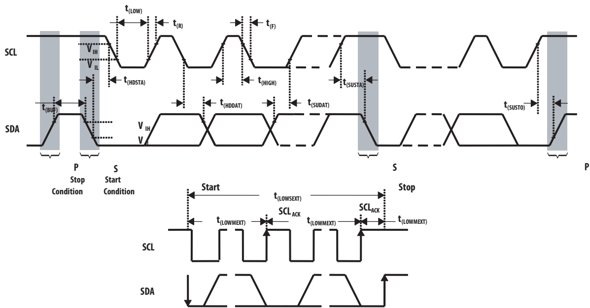
Figure 1. Timing Diagrams
