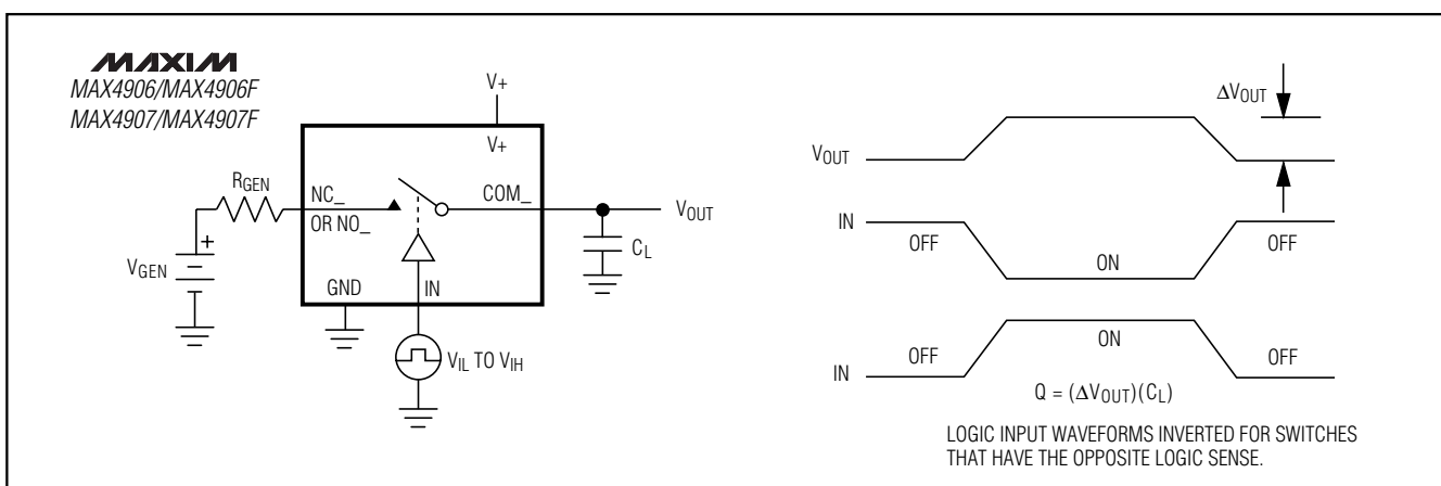
Figure 6. Charge Injection
