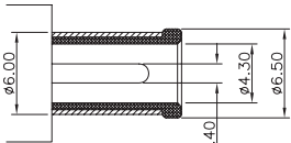
MATING PLUG Jack Insertion Depth: 9.1 mm
