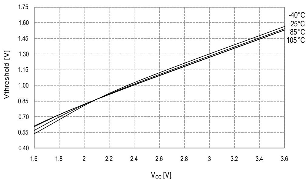
Figure 34-113. I/O Pin Input Threshold Voltage vs. V_{CC} V_{IL} I/O pin read as "0"
