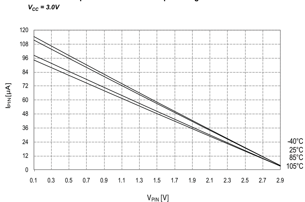
Figure 34-101. I/O Pin Pull-up Resistor Current vs. Input Voltage
