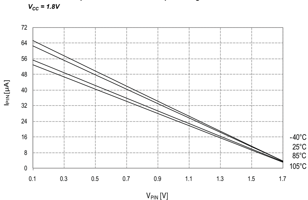
Figure 34-100. I/O Pin Pull-up Resistor Current vs. Input Voltage
