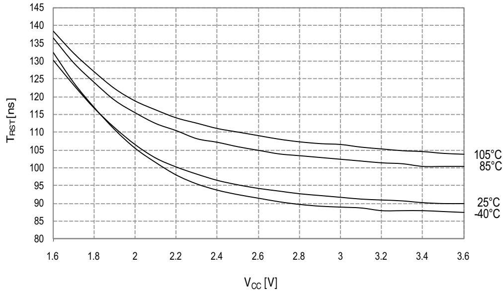
Figure 34-136. Minimum Reset Pin Pulse Width vs. V_{CC}
