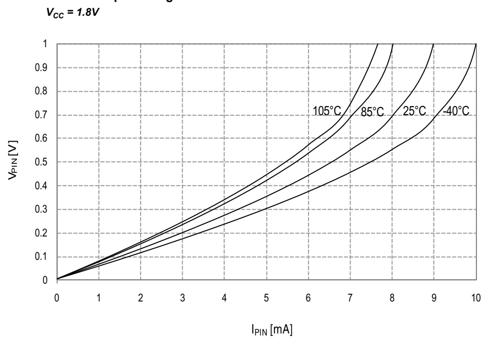
Figure 34-28. I/O Pin Output Voltage vs. Sink Current
