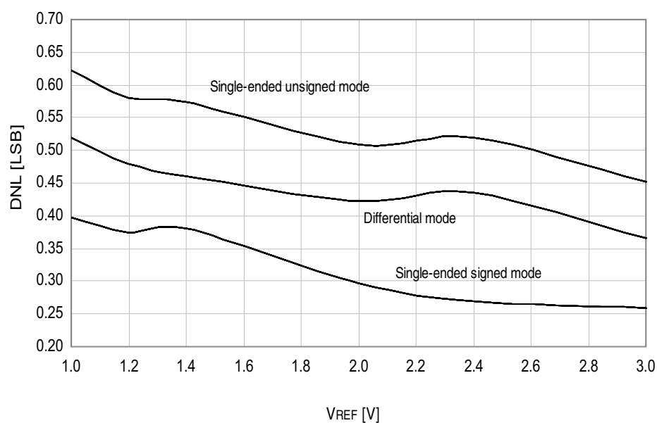
Figure 34-118. DNL Error vs. External V_{REF} T = 25^{\circ}\text{C} , V_{CC} = 3.6\text{V} , external reference
