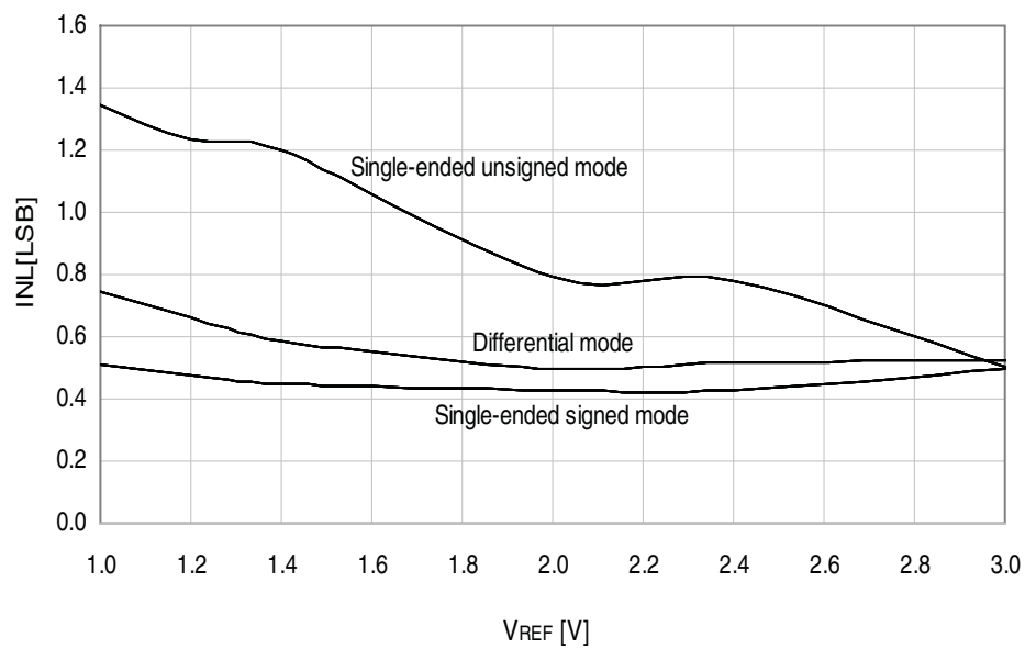
Figure 34-115. INL Error vs. External V_{REF} T = 25^\circ\text{C} , V_{CC} = 3.6\text{V} , external reference
