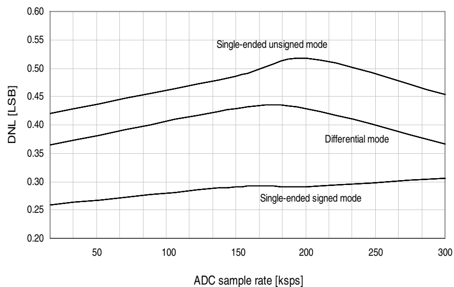
Figure 34-119. DNL Error vs. Sample Rate T = 25^{\circ}\text{C} , V_{CC} = 3.6\text{V} , V_{REF} = 3.0\text{V} external
