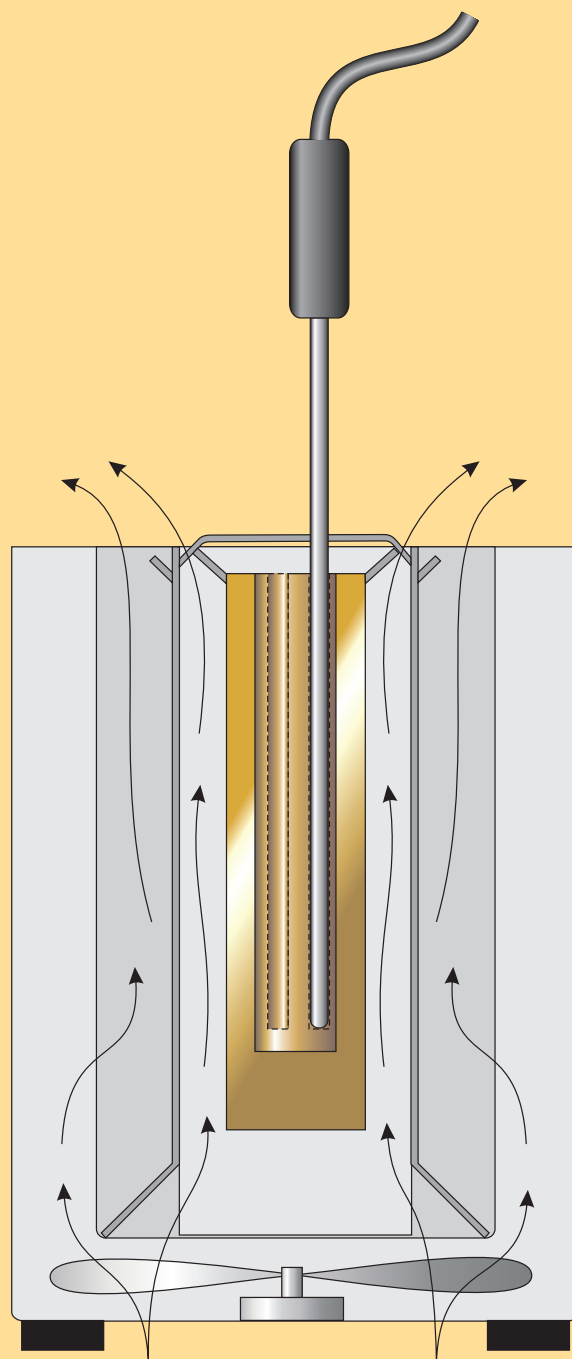
Simplified schematic illustrating the airflow design (patents applied for) to minimize potential heat damage to sensor handles and transition junctions.
