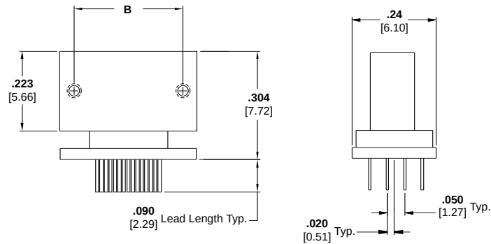
Receptacle Assembly Drawing Number 1589488
