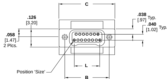
Plug Assembly Drawing Number 1589482
