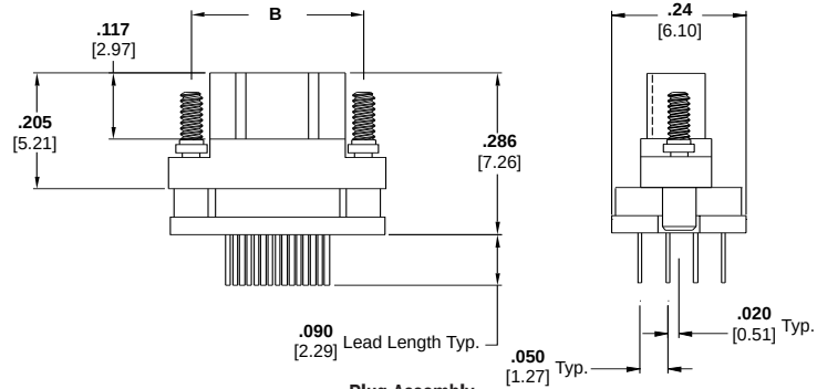
Plug Assembly Drawing Number 1589482
