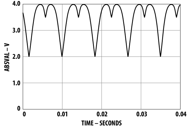
Figure 23. ABSVAL with 2 phases, wired-ORed together.
