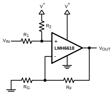
Figure 68. DC Level Shifting
