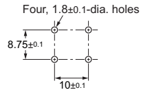
PCB Dimensions (Bottom View)
