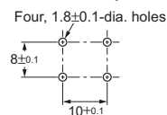
PCB Dimensions (Bottom View)
