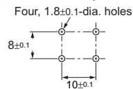
PCB Dimensions (Bottom View)
