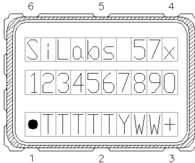
Figure 7. Mark Specification
