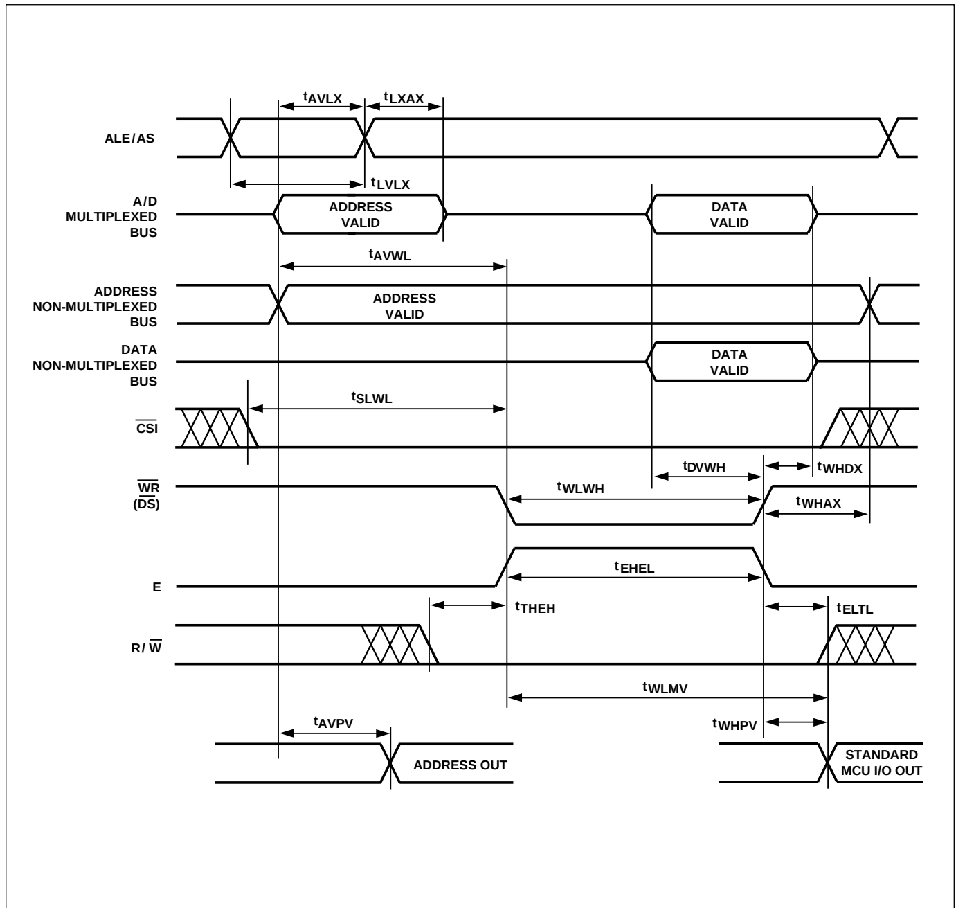
Figure 28. Write Timing
