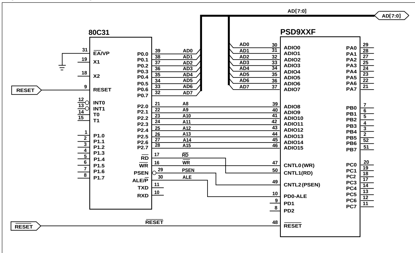
Figure 14. Interfacing the PSD9XX with an 80C31
