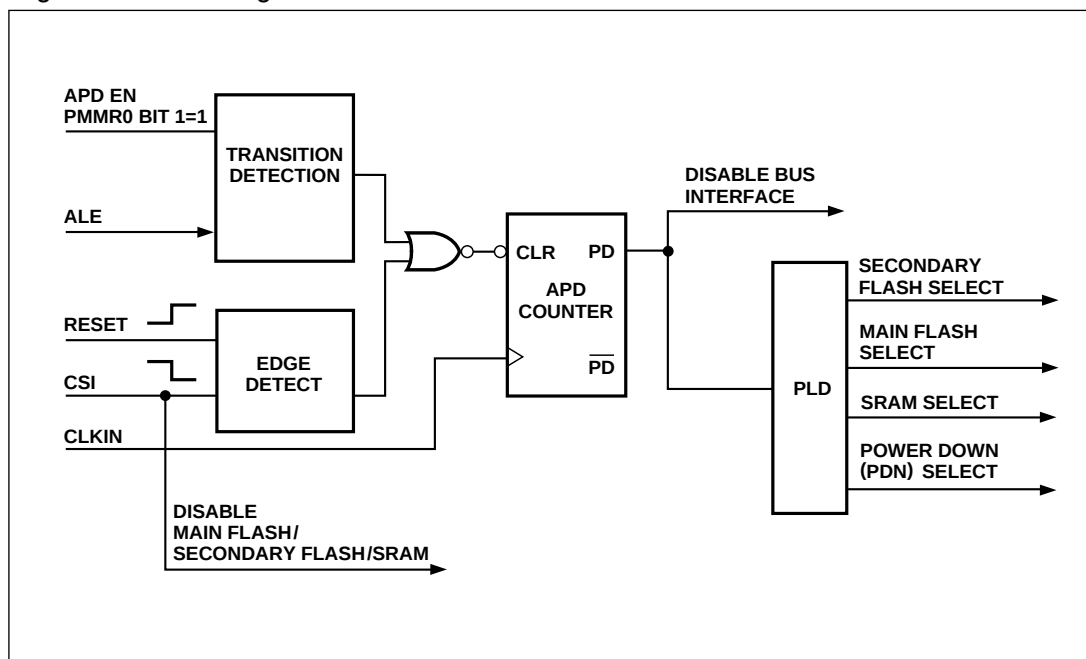
Figure 23. APD Logic Block
