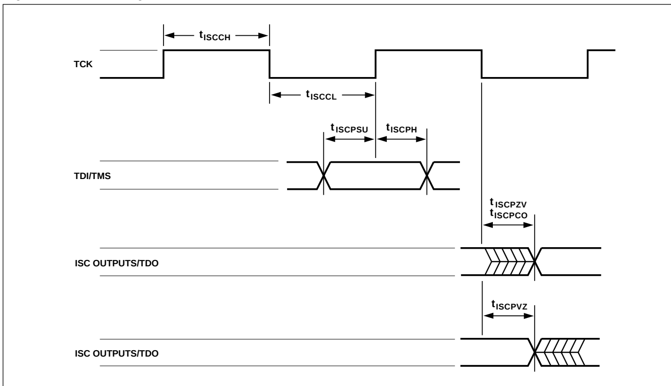
Figure 30. ISC Timing
