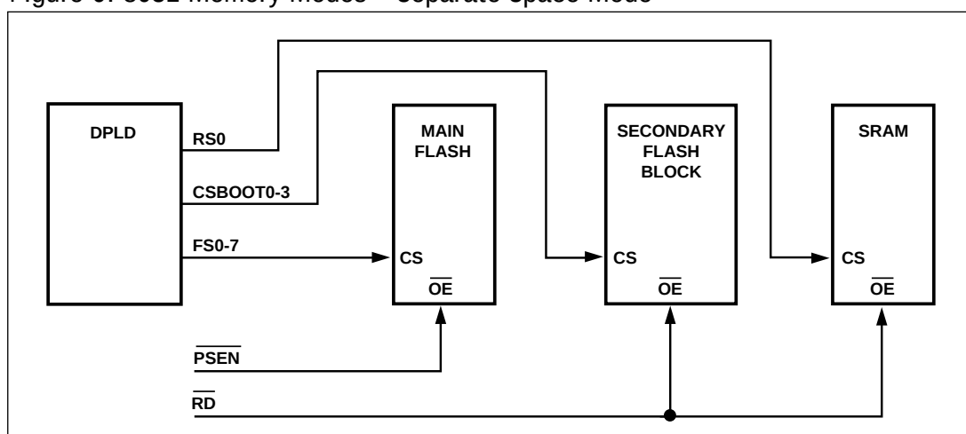
Figure 6. 8031 Memory Modes – Separate Space Mode
