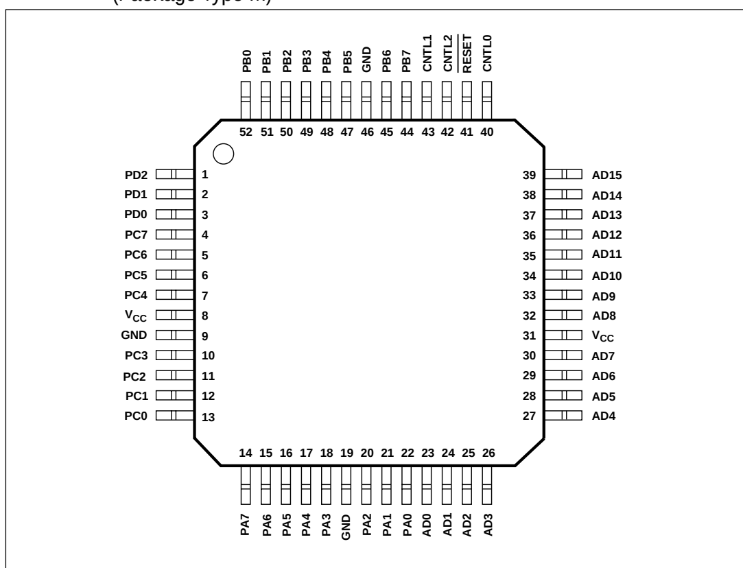
Figure 36. Drawing M3 – 52-Pin Plastic Quad Flatpack (PQFP) (Package Type M)
