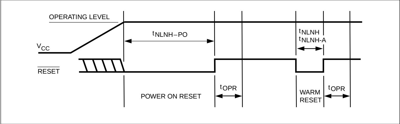
Figure 31. Reset Timing
