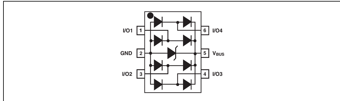
Figure 1. Functional diagram
