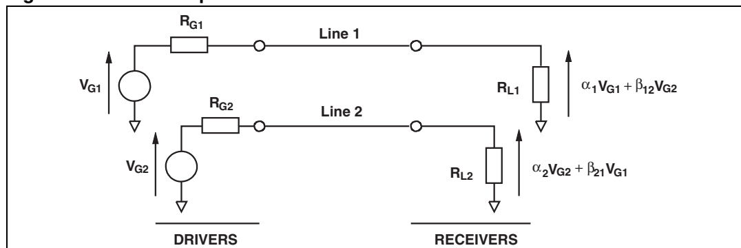
Figure 15. Crosstalk phenomena
