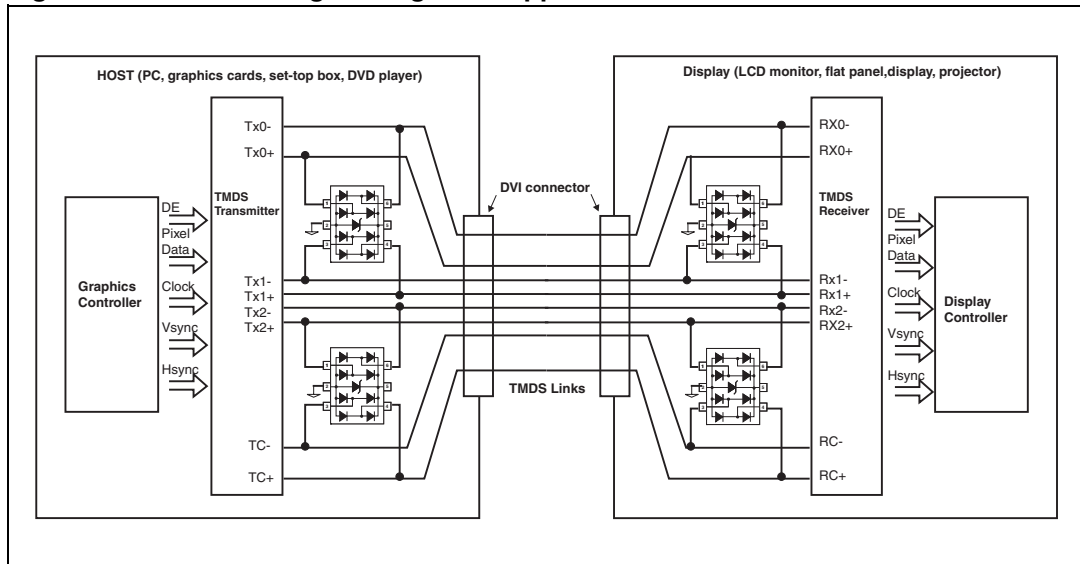
Figure 9. DVI/HDMI digital single link application
