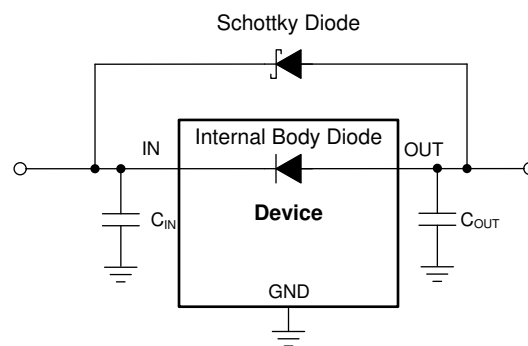
Figure 6-7. Example Circuit for Reverse Current Protection Using a Schottky Diode
