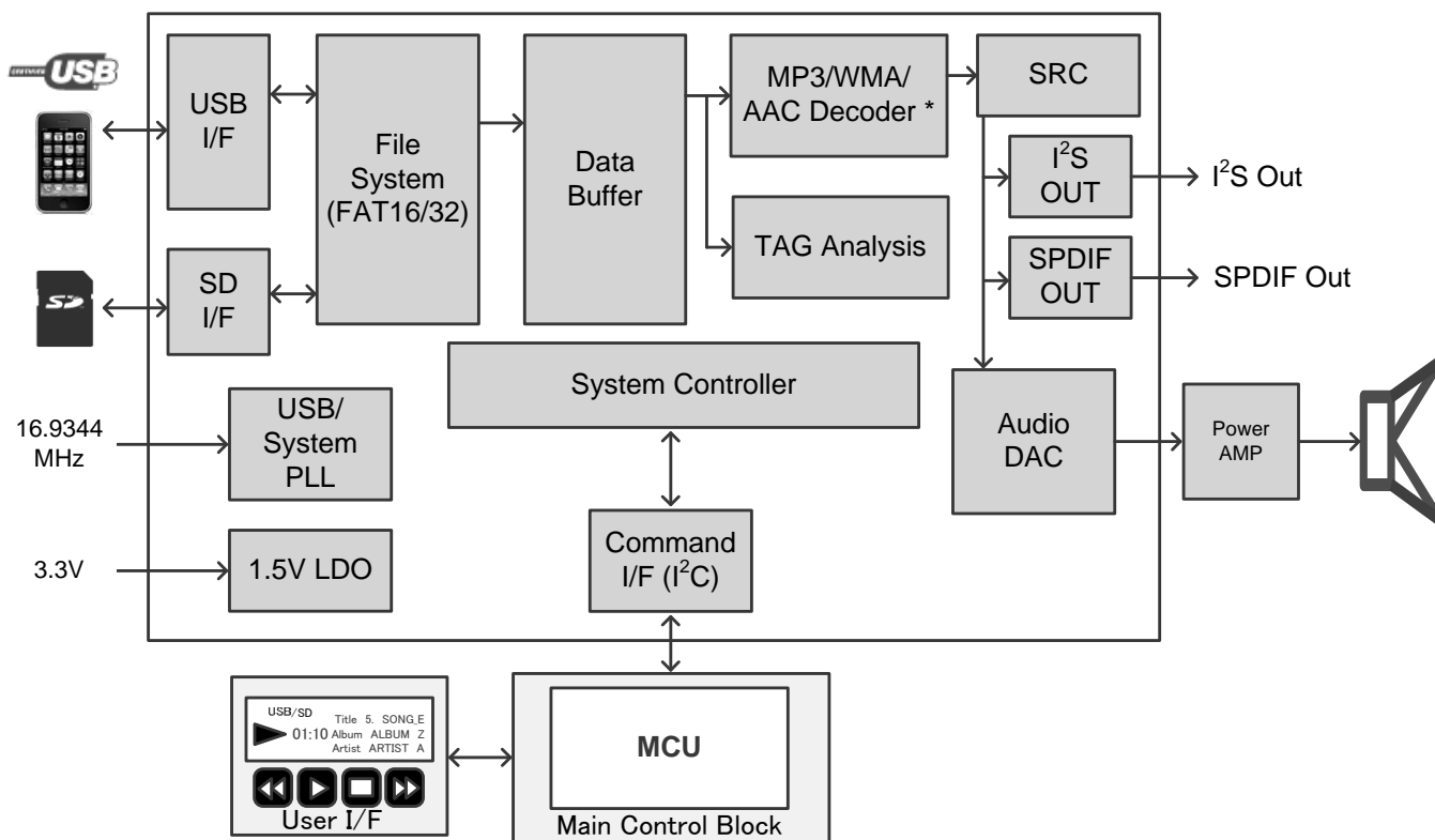
Figure 4. Block diagram
