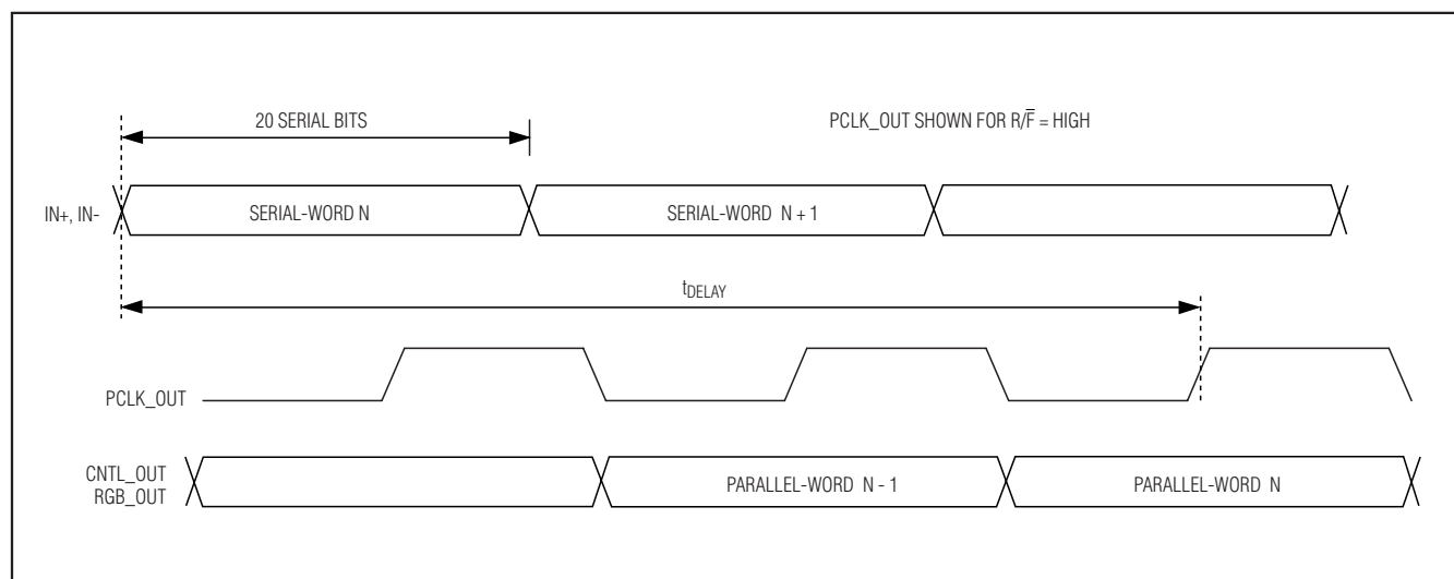
Figure 6. Deserializer Delay
