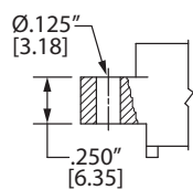
CLEARANCE HOLE (H)
