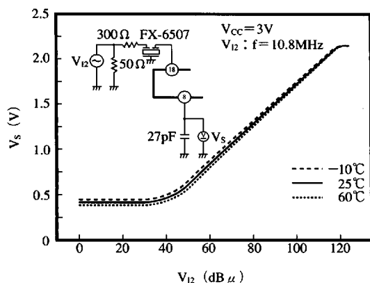
RSSI Output Voltage—IF Input Level
