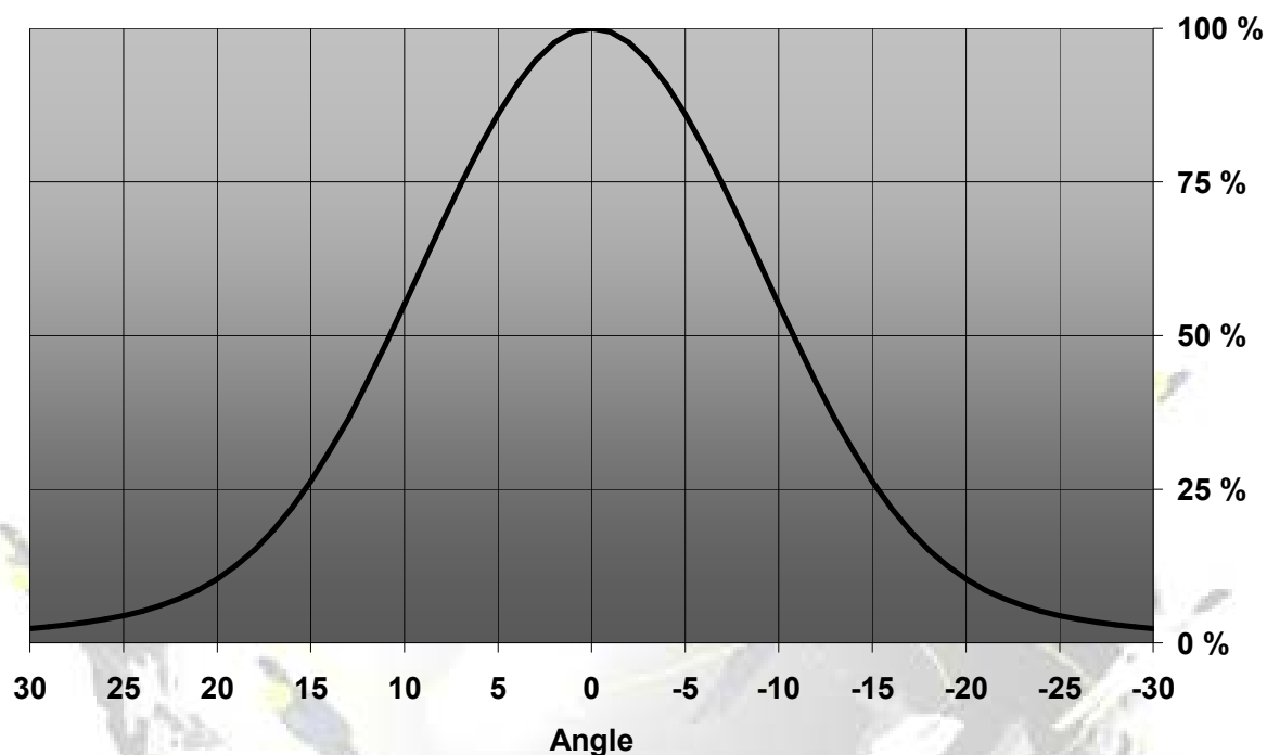
Relative Intensity of Lisa-R1-SS
