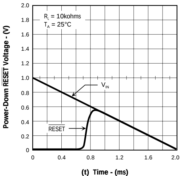
FIGURE 3. — POWER-DOWN RESET VOLTAGE
