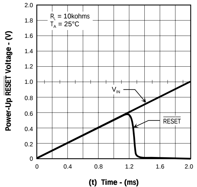
FIGURE 2. — POWER-UP RESET VOLTAGE
