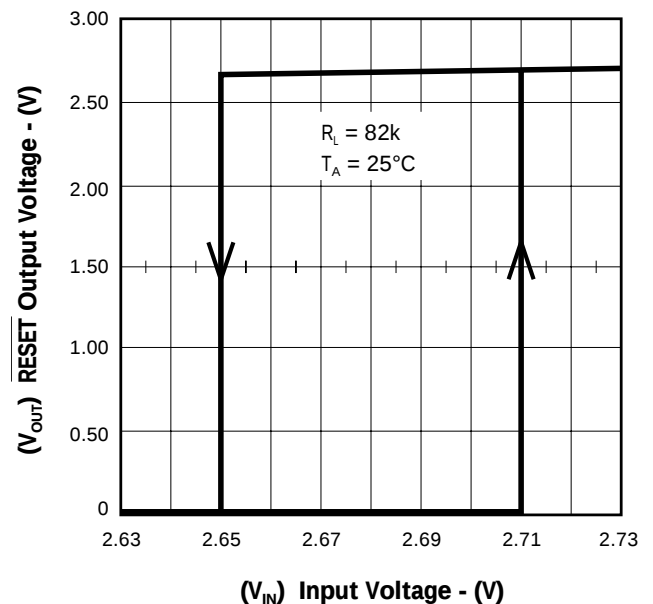
FIGURE 4. — RESET OUTPUT VOLTAGE vs. INPUT VOLTAGE
