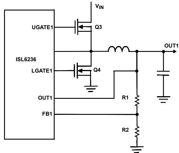
FIGURE 76. SETTING V_{OUT1} WITH A RESISTOR DIVIDER
