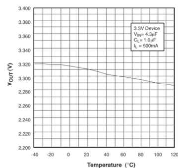
Fig. 14 Output Voltage vs Temperature
