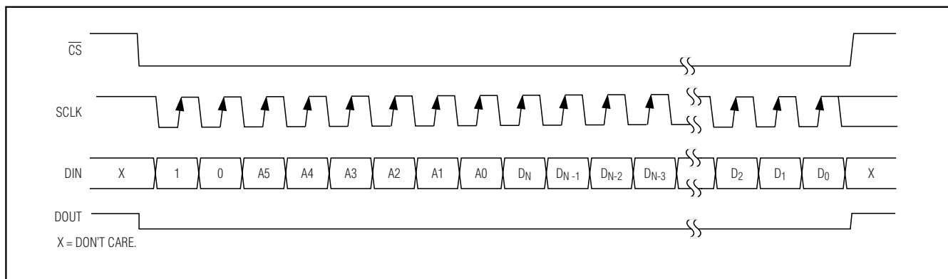
Figure 16. Serial-Interface Register Write with 8-Bit Control Word, Followed by a Variable Length Data Write
