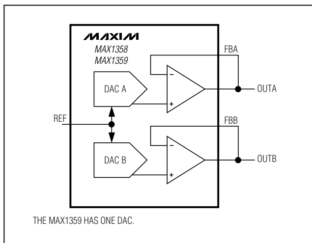
Figure 24. DAC Unipolar Output Circuit
