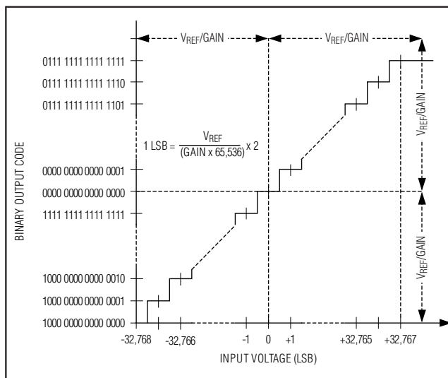
Figure 23. ADC Bipolar Transfer Function
