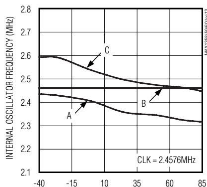
INTERNAL OSCILLATOR FREQUENCY vs. TEMPERATURE
