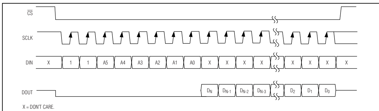
Figure 17. Serial-Interface Register Read with 8-Bit Control Word Followed by a Variable Length Data Read
