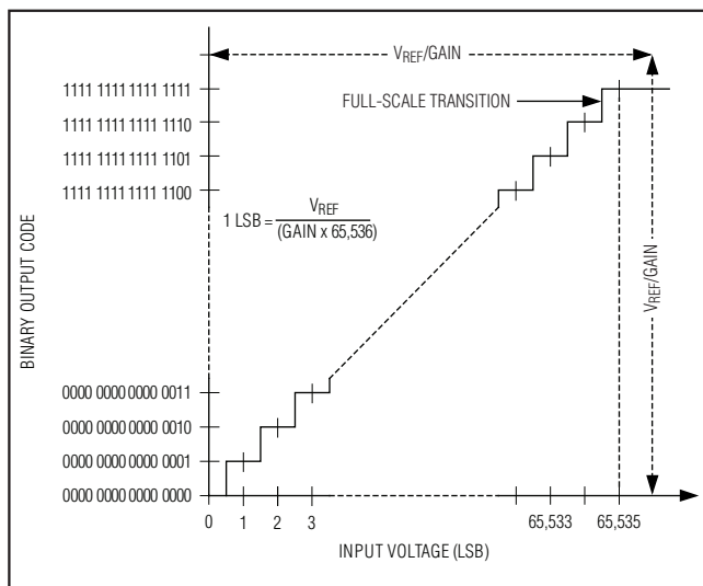
Figure 22. ADC Unipolar Transfer Function
