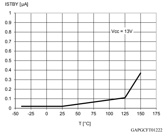
Figure 16. Standby current
