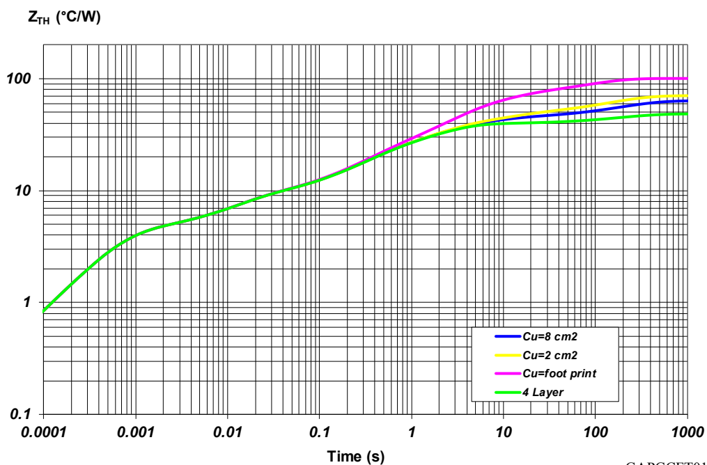
Figure 44. SO-8 thermal impedance junction ambient single pulse (one channel on)
