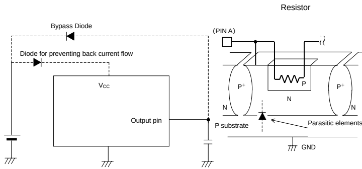
Fig.23 Bypass Diode
