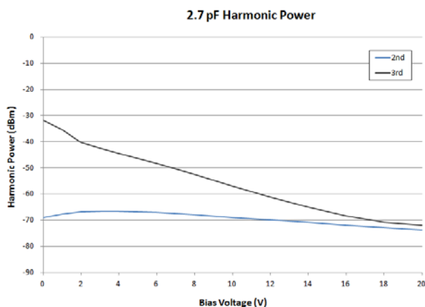
Figure 3. Harmonic Power*
