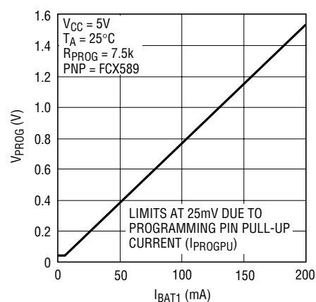
Program Pin Voltage vs Charge Current (200mA)
