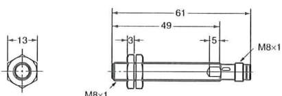
E2A-S08LS02-M5-□□
