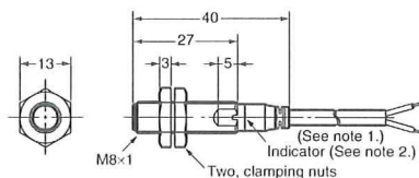
E2A-S08KS02-WP-□□
