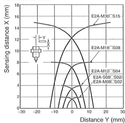
Shielded Models
