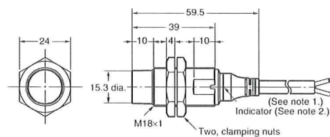
E2A-M18KN16-WP-□□
