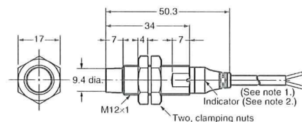
E2A-M12KN08-WP-□□
