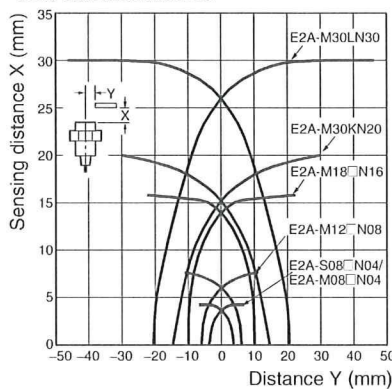
Non-shielded Models
