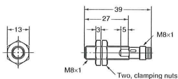
E2A-S08KS02-M5-□□
