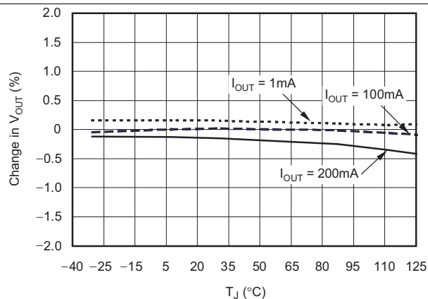
Figure 1. Load Regulation
