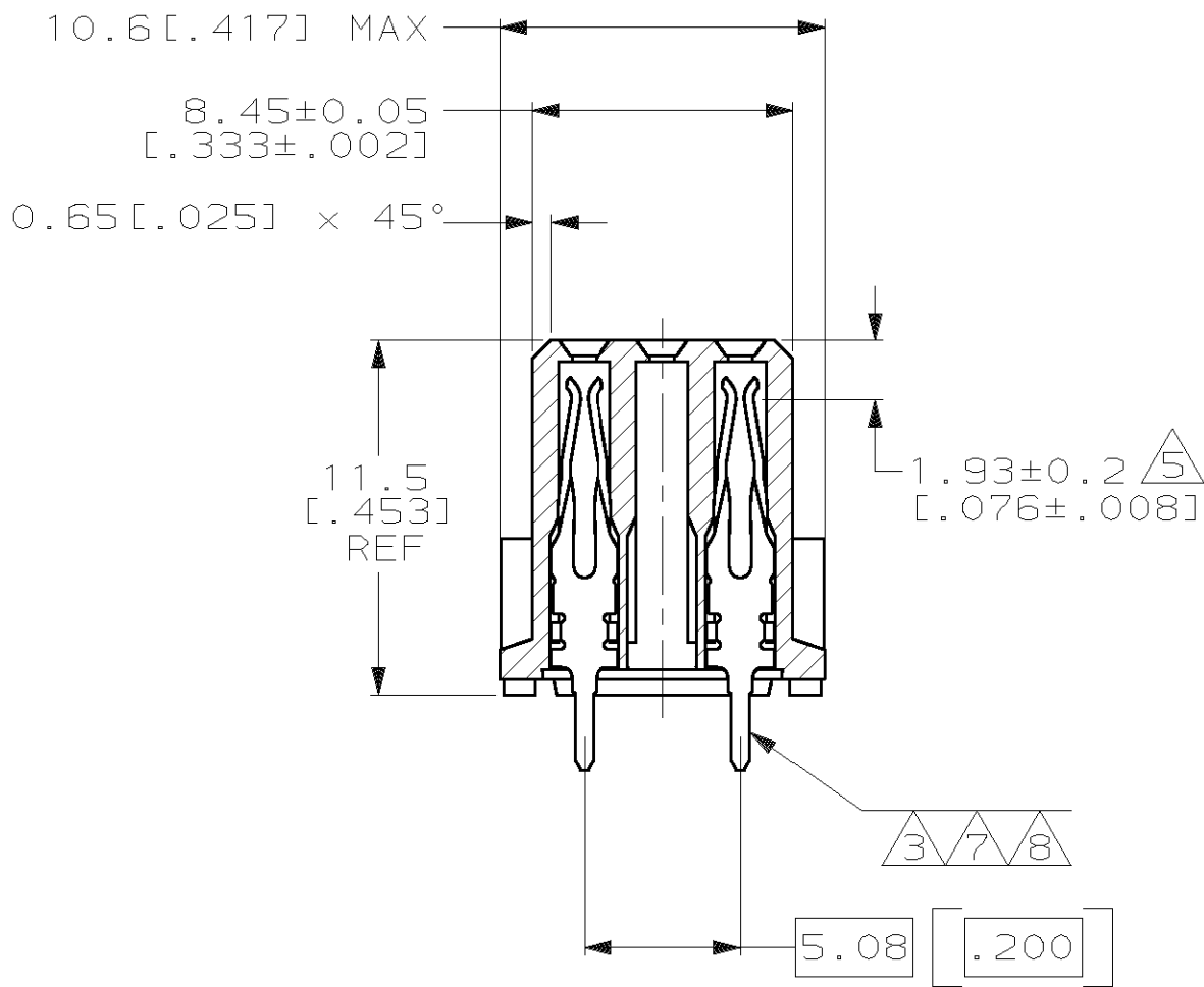
SECTION X-X
