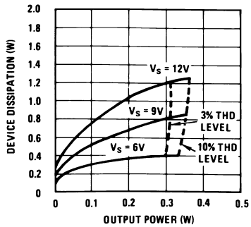
Device Dissipation vs Output Power—4 \Omega Load
