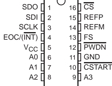
TLV2544Q . . . D PACKAGE (TOP VIEW)
