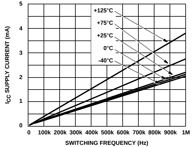
FIGURE 7. I_{CC0} , NO-LOAD I_{CC} SUPPLY CURRENT vs FREQUENCY (Hz) TEMPERATURE
