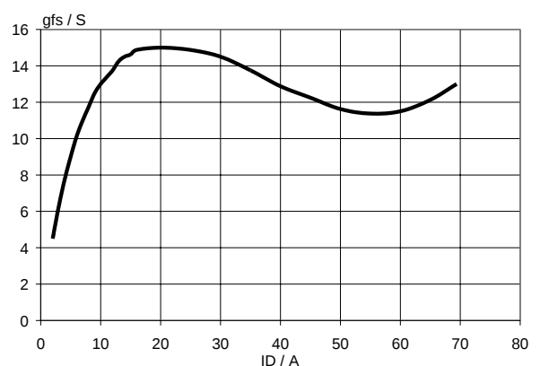
Fig.9. Typical transconductance, T_j = 25\text{ °C} . g_{fs} = f(I_D) ; conditions: V_{DS} = 25\text{ V}
