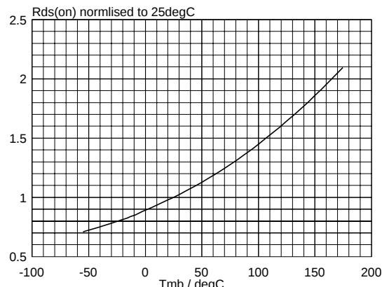
Fig.10. Normalised drain-source on-state resistance. a = R_{DS(ON)}/R_{DS(ON)25\text{ °C}} = f(T_j) ; I_D = 25\text{ A} ; V_{GS} = 5\text{ V}
