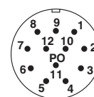
M23 plug connection pin, 12-pos.
