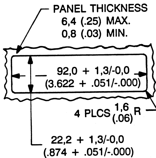
PANEL CUTOUT
