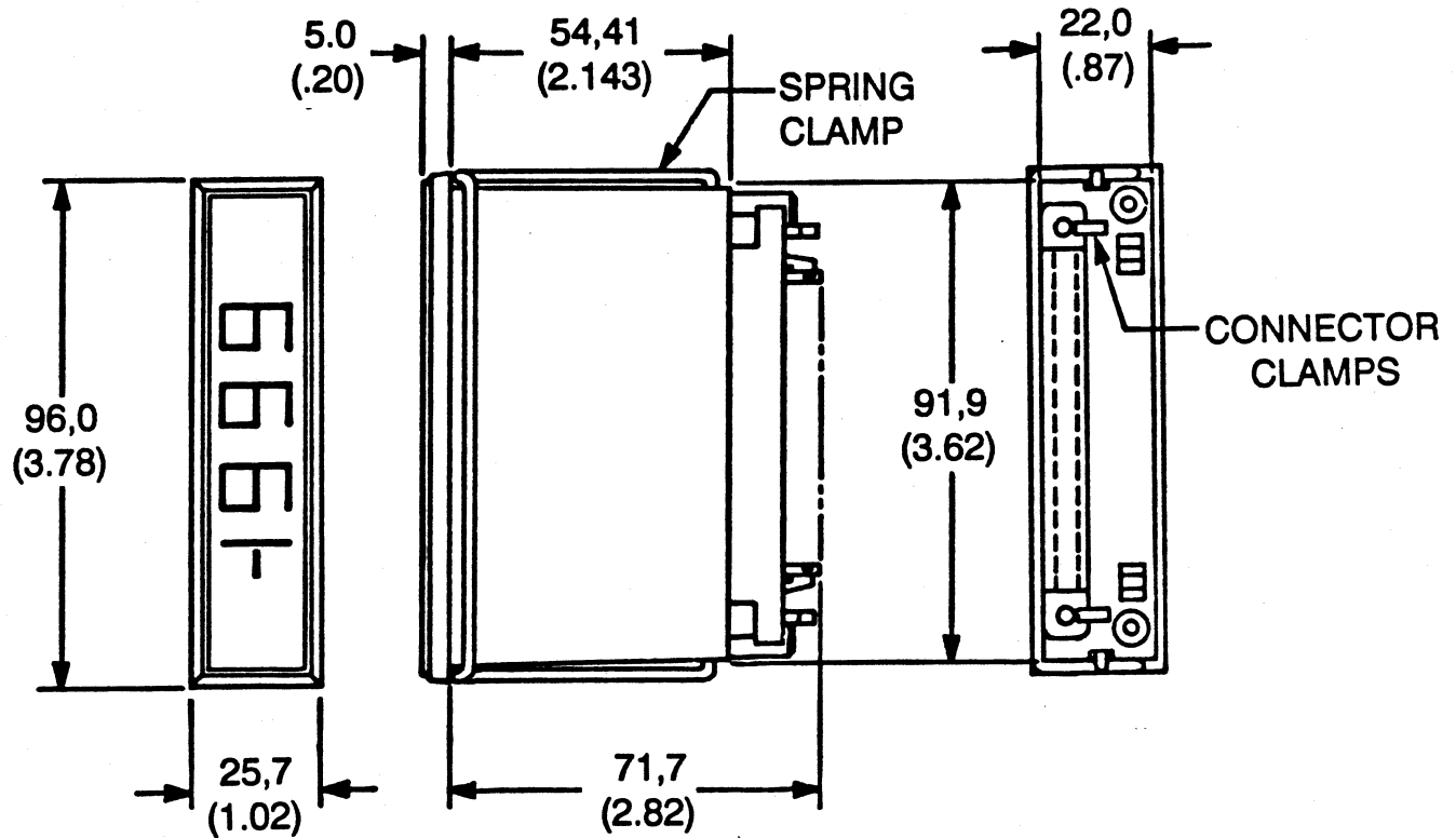
REAR VIEW
