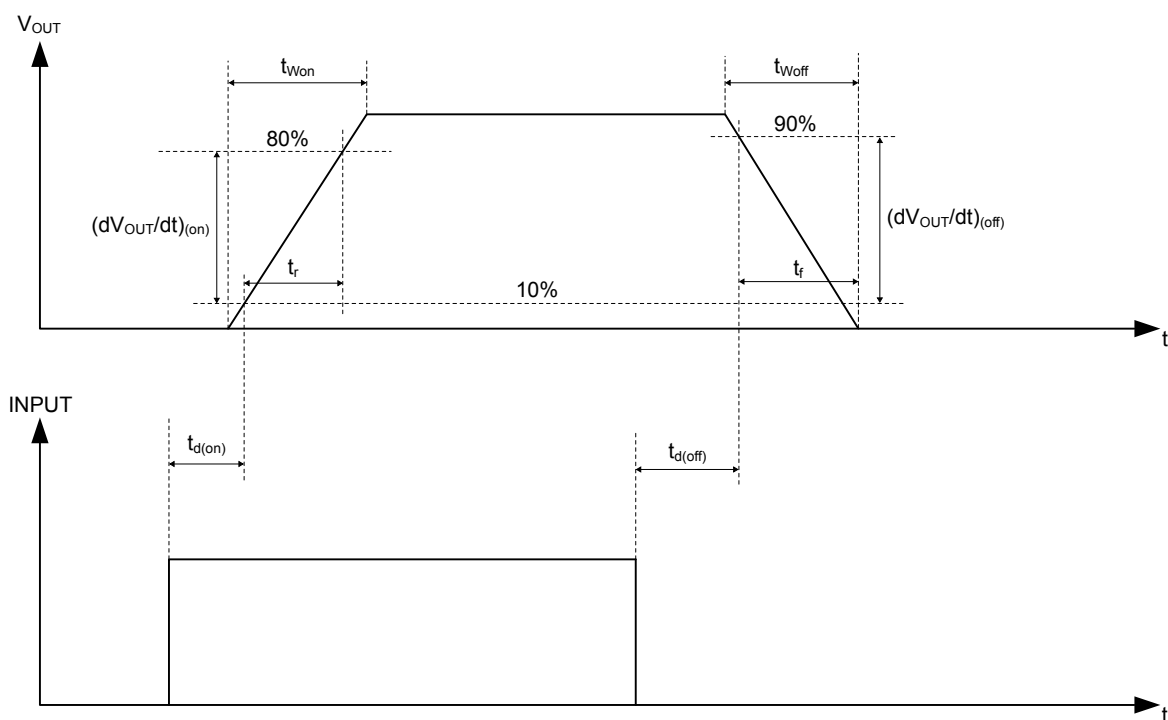
Figure 8. Switching characteristics
