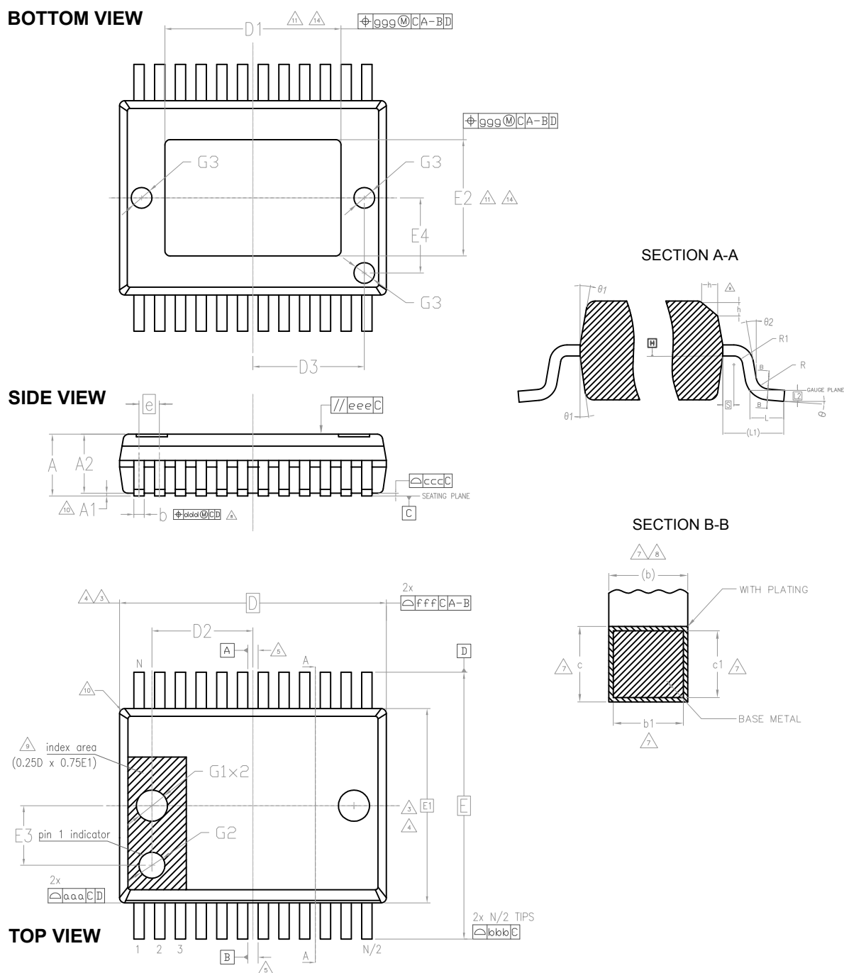
Figure 30. PowerSSO-24 package dimensions
