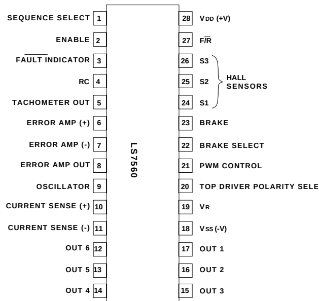
FIGURE 1. PIN CONNECTION DIAGRAM TOP VIEW
