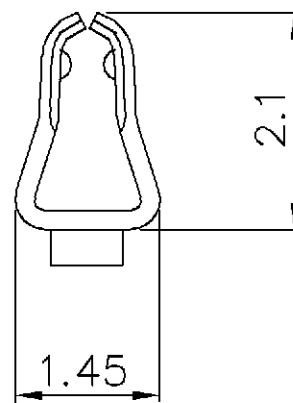
SEC C-C
