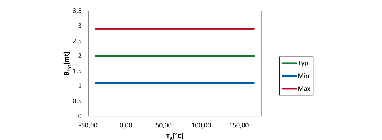
Figure 5-3 Hysteresis ( B_{Hys} ) of the TLE4968-1L over Temperature
