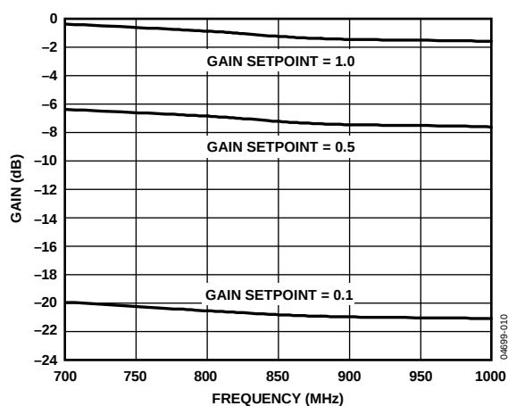
Figure 10. Gain vs. Frequency at Different Gain Setpoints (700 MHz to 1000 MHz), Phase Setpoint = 0^\circ
