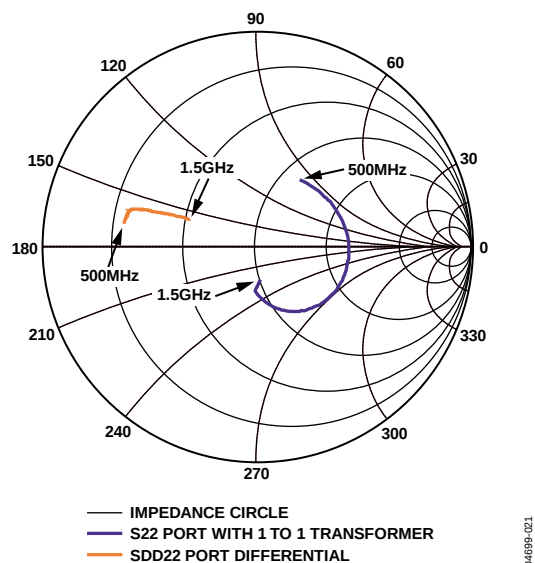
Figure 21. Output Impedance Smith Chart (with Frequency Markers)
