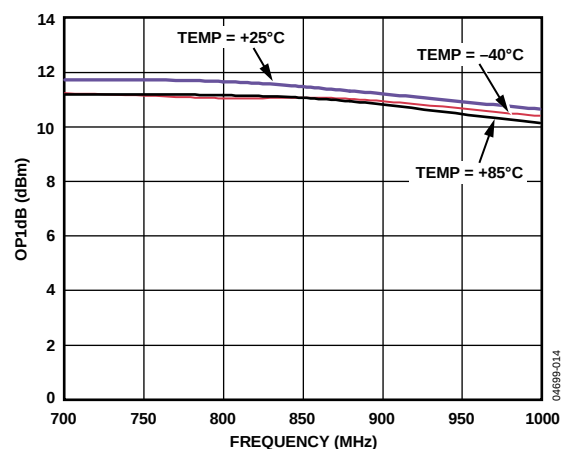
Figure 14. Output 1 dB Compression Point vs. Frequency and Temperature, Maximum Gain, Phase Setpoint = 0^\circ
