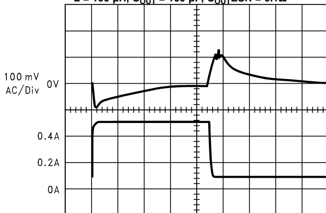
Load Transient Response for Continuous Mode V_{IN} = 20V , V_{OUT} = 5V L = 100\text{ }\mu\text{H} , C_{OUT} = 100\text{ }\mu\text{F} , C_{OUT}ESR = 0.1\Omega
