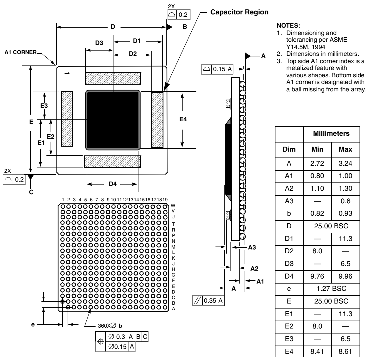
Figure 13. Mechanical Dimensions and Bottom Surface Nomenclature for the MPC7447A, 360 HCTE BGA Package
