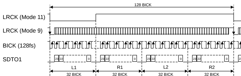
Figure 17. Mode 9/11 Timing (TDM128 mode, I 2 S Compatible)
