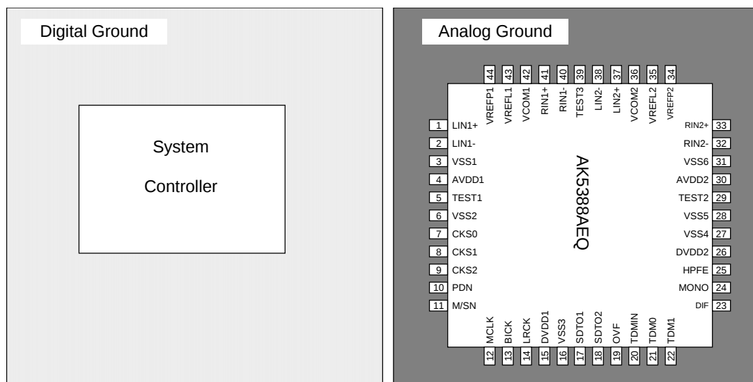
Figure 24. Ground Layout
