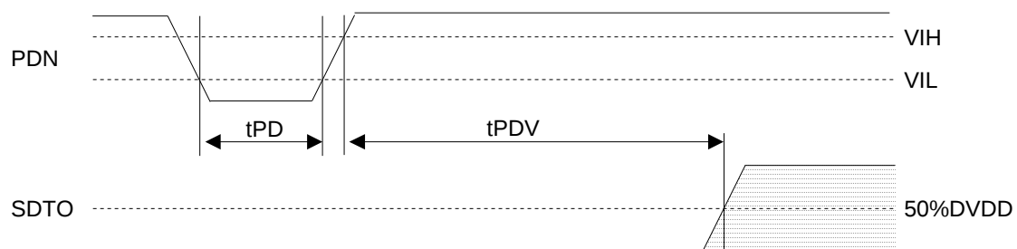
Figure 9. Power Down &amp; Reset Timing
