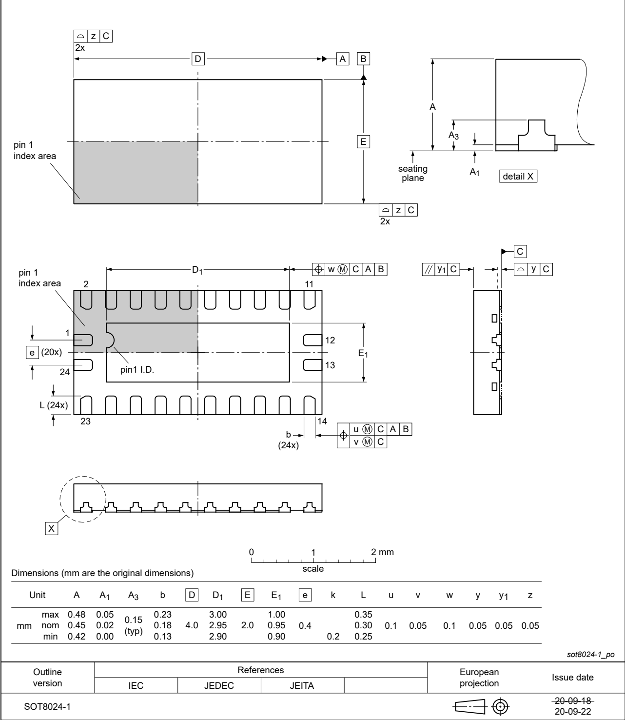
Fig. 12. Package outline SOT8024-1 (DHXQFN24)
