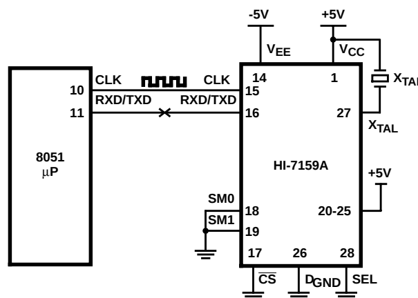
FIGURE 4A. SERIAL MODE 0
