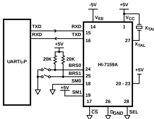
FIGURE 4B. SERIAL MODE 1
