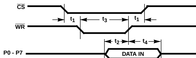
FIGURE 1A. WRITE
