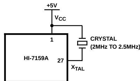
FIGURE 7. SINGLE-PIN OSCILLATOR
