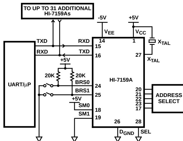
FIGURE 4C. SERIAL MODE 2
