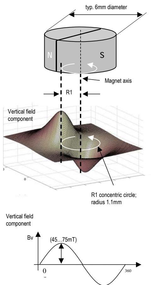
Figure 16: Typical magnet (6x3mm) and magnetic field distribution
