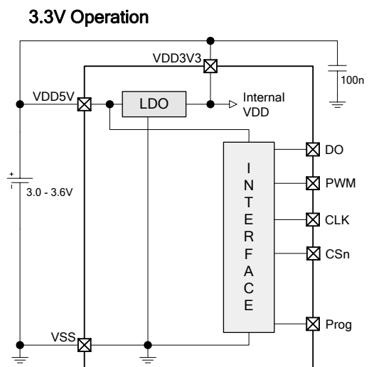
Figure 15: Connections for 5V / 3.3V supply voltages
