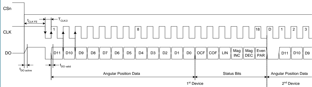
Figure 6: Daisy Chain mode data transfer
