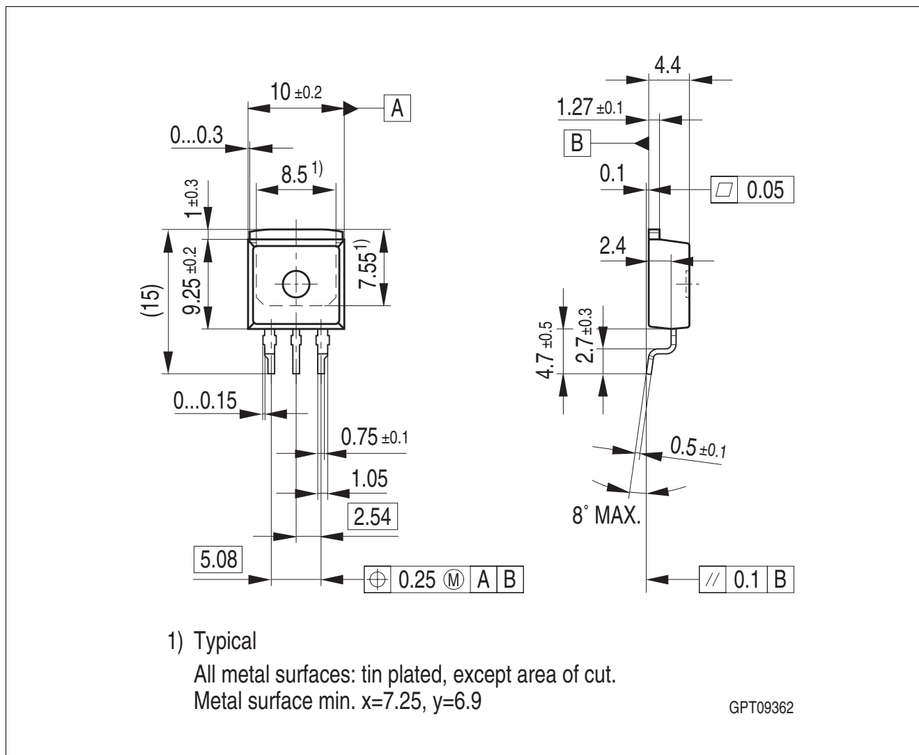
Figure 4 PG-TO263-3
