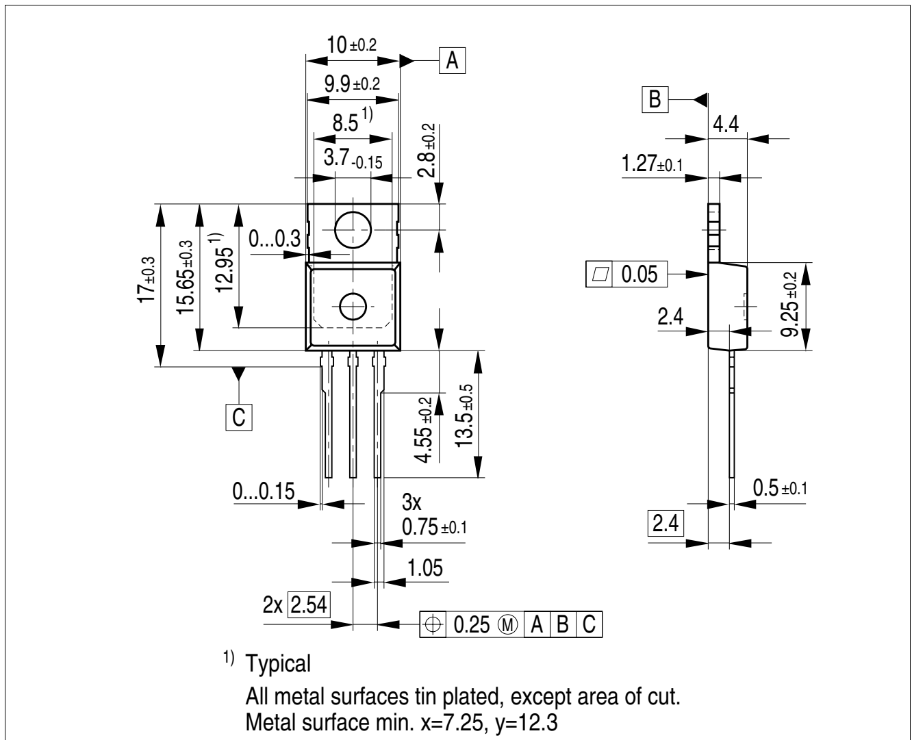
Figure 5 PG-T0220-3
